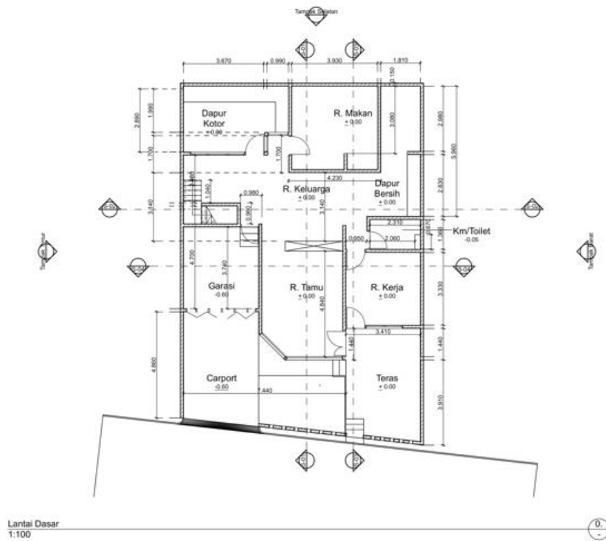
Figure 1. Existing Plan
