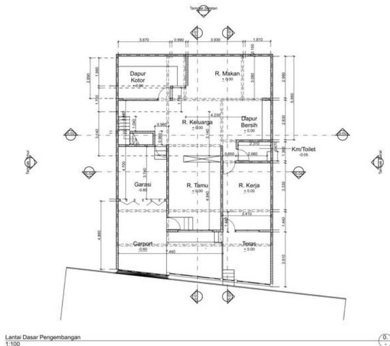
Figure 2. Renovation Plan
