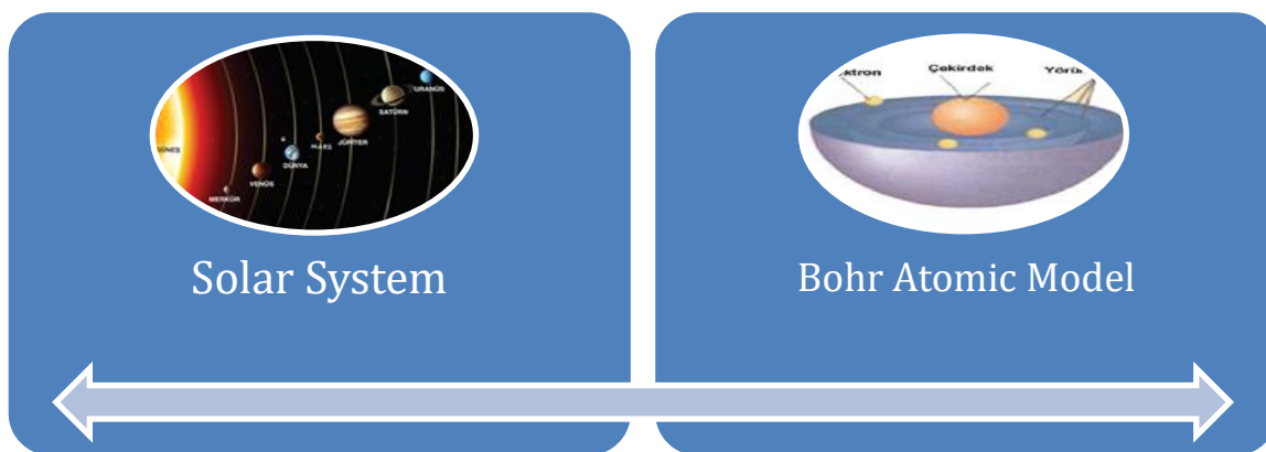
Image 1 Solar system
